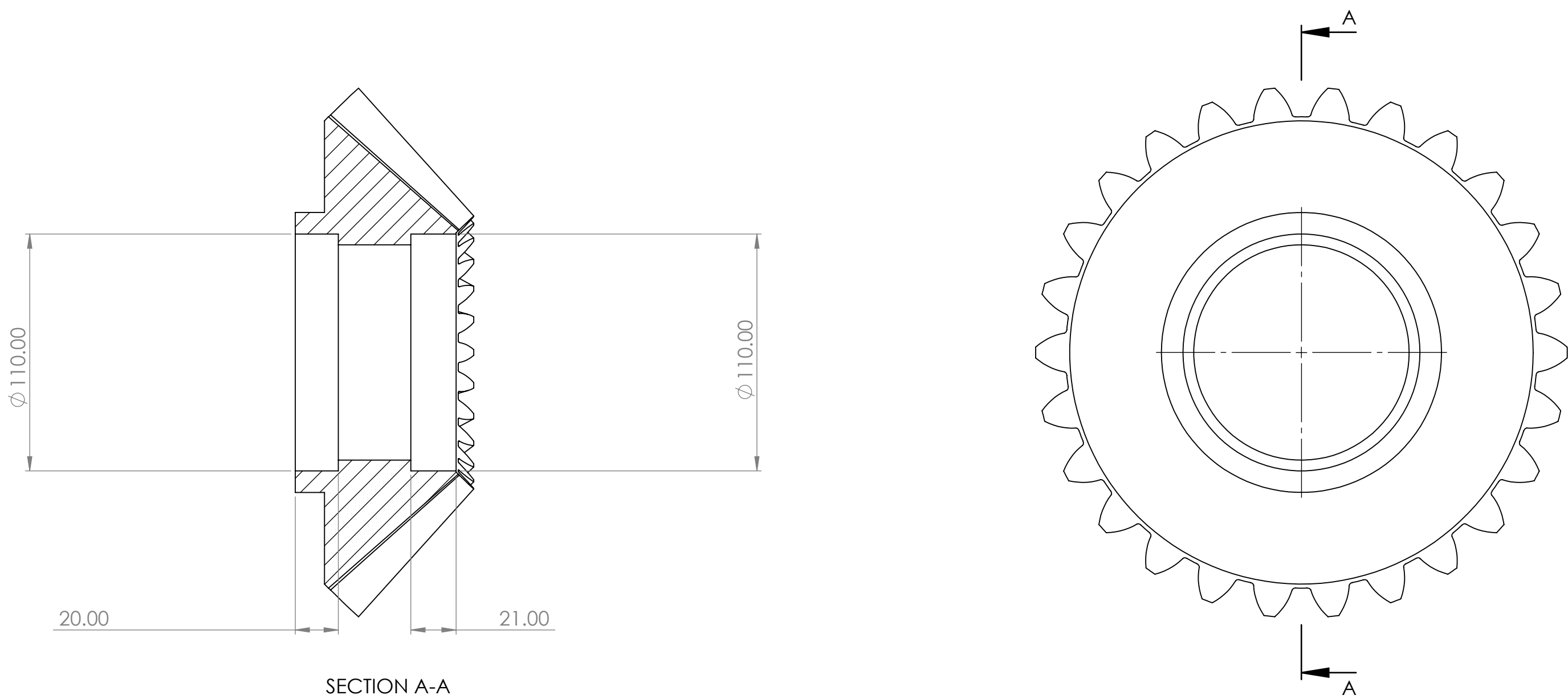
Part5 spider gear
