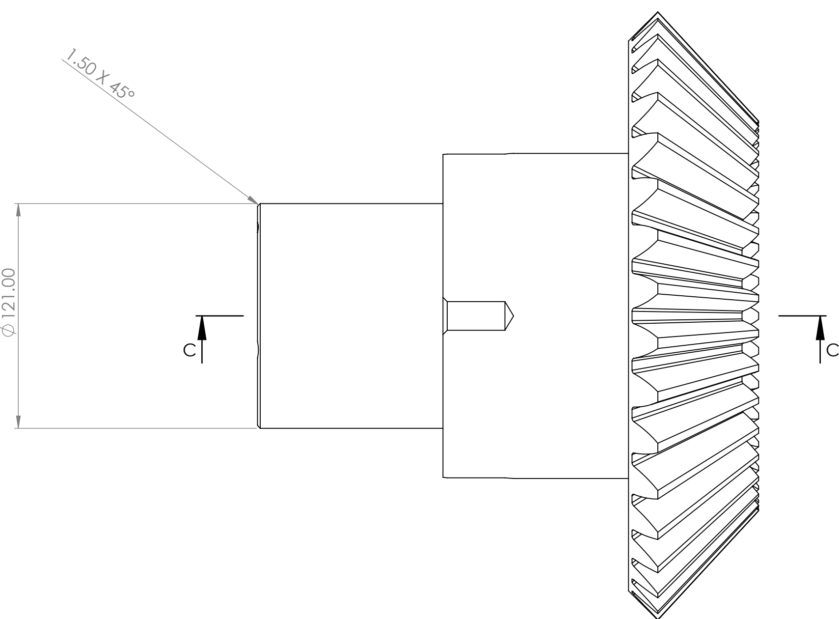
Part3 side gear B
