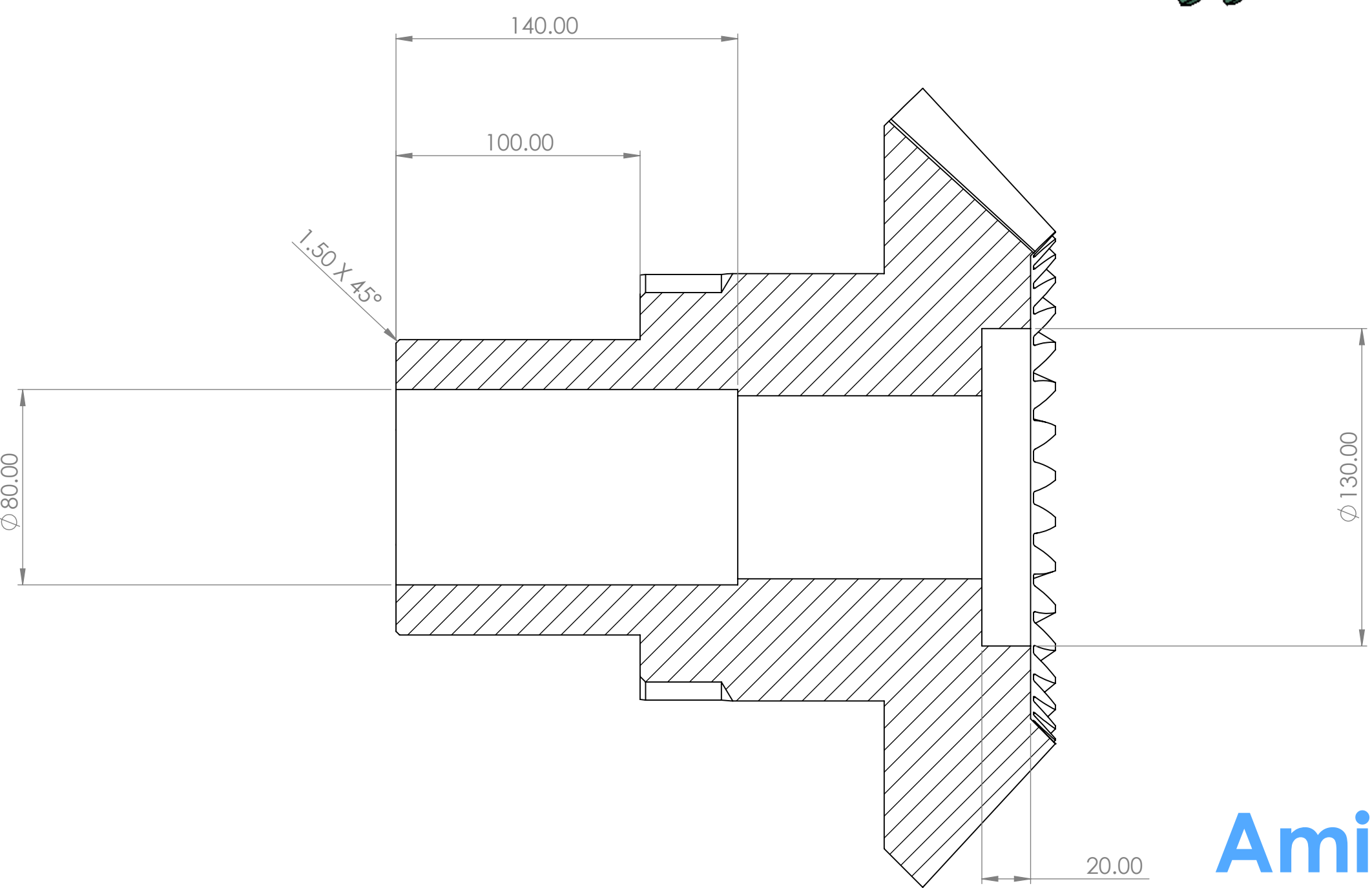
SECTION C-C
